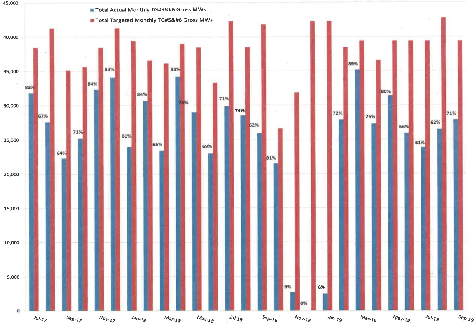
Combined Monthly TG#5&#6 Gross MWs -Actual to Targeted
